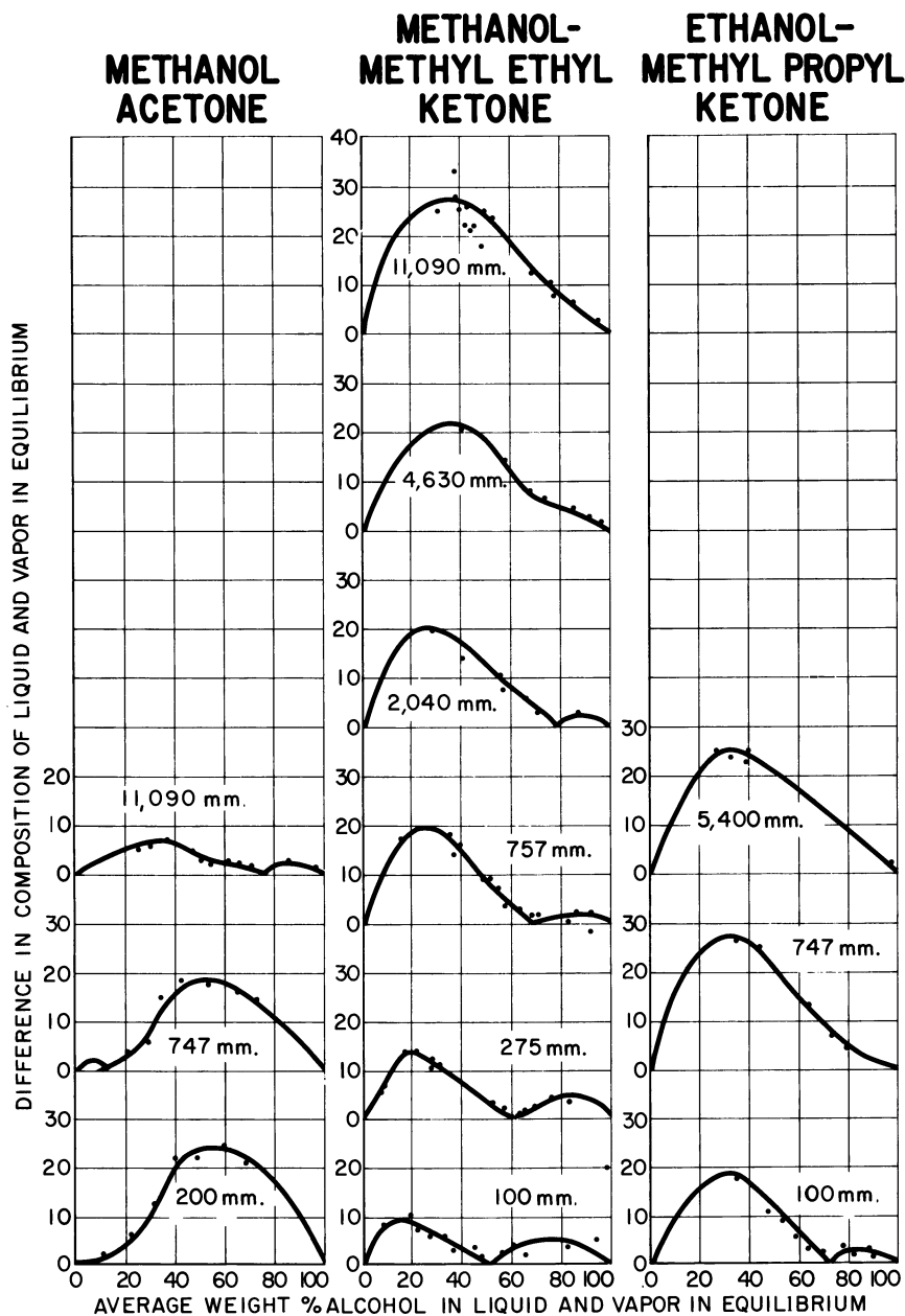
Figure 2. Difference in composition of vapor and liquid in equilibrium
