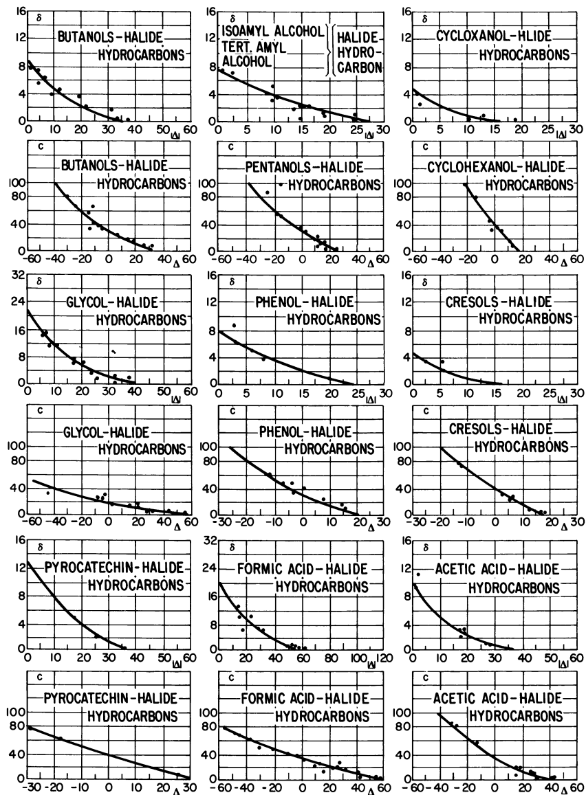
Figure 3. C-Δ and δ-|Δ| curves for alcohol-halide hydrocarbon, glycol-halide hydrocarbon, phenol-halide hydrocarbon, and acid-halide hydrocarbon systems
